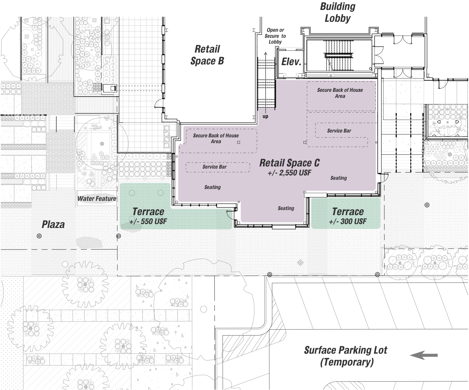
Floor Plan
