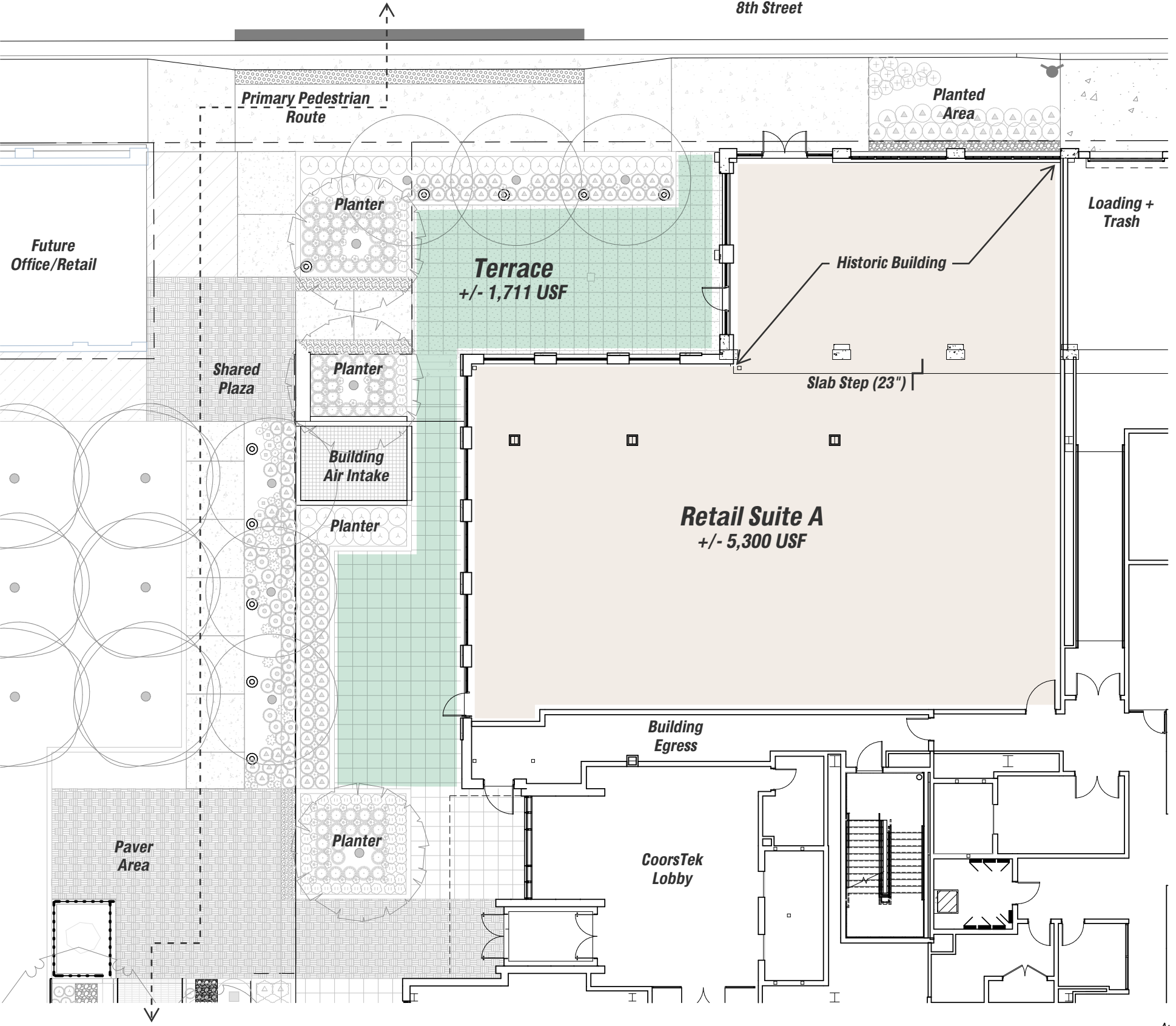
Floor Plan
